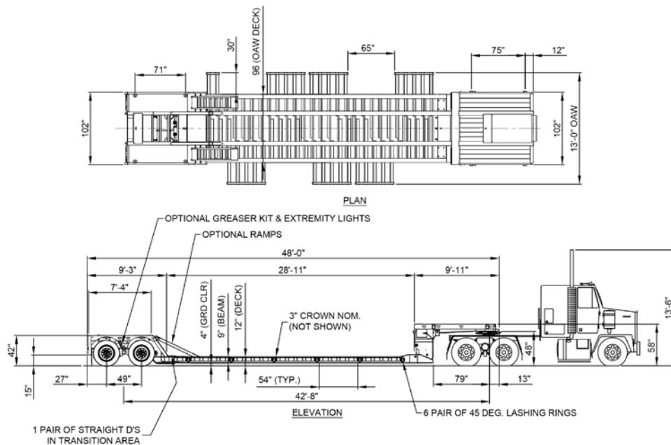
MODEL: 35ADG2X48 AGULP 35TON AIR DETACHABLE GOOSENECK, 2 AXLE, 48 FT., AGRI, ULTRA LOW PRO NOTE: ALL DIMENSIONS ARE LOADED & NOMINAL.
