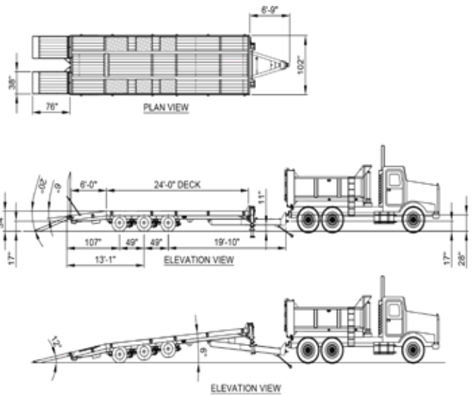
MODEL: 25ART 25 TON, AIR RAMP, AIR TILT, TAG NOTE: ALL DIMENSIONS ARE LOADED & NOMINAL.
