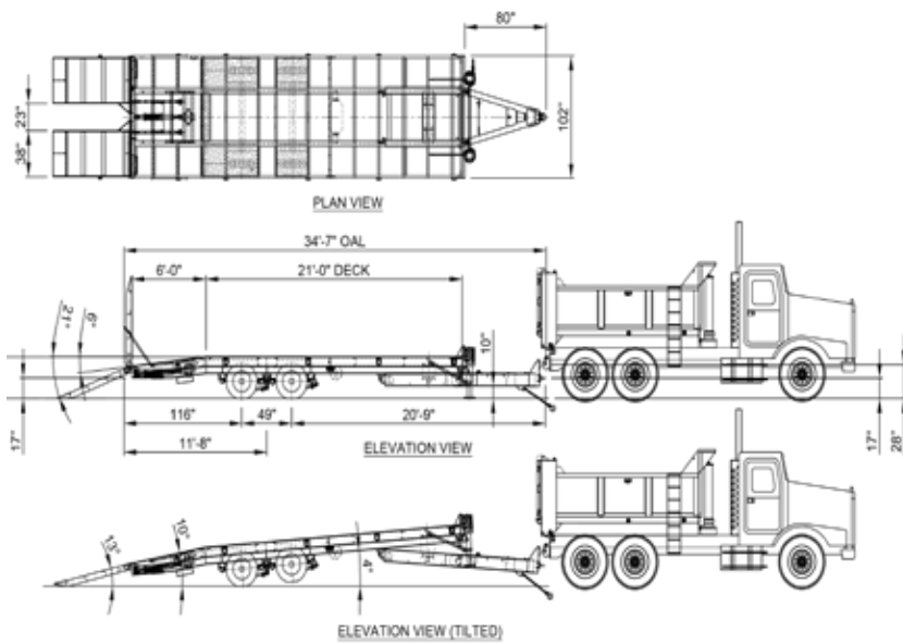
MODEL: 20ART 20 TON TANDEM AIR TILT/AIR RAMP NOTE: ALL DIMENSIONS ARE LOADED & NOMINAL.
