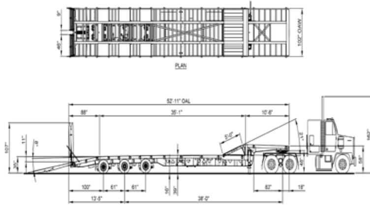
ELEVATION MODEL: 53ET3XP 53FT. TRIDEM
