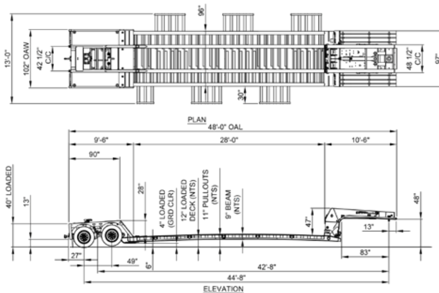
MODEL: 35HDG2X48 AGULP 35 TON HYDRAULIC DETACHABLE GOOSENECK 2 AXLE, 48 FT., AGRI, ULTRA LOW PRO NOTE: ALL DIMENSIONS ARE LOADED & NOMINAL.
