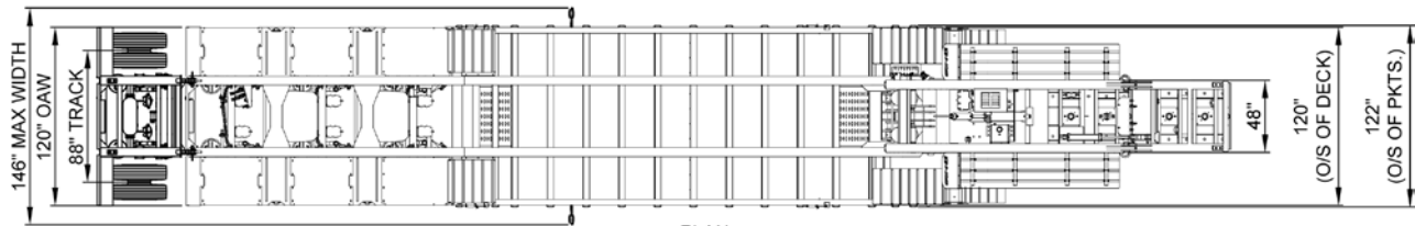
PLAN 58'-4" TOTAL OAL
