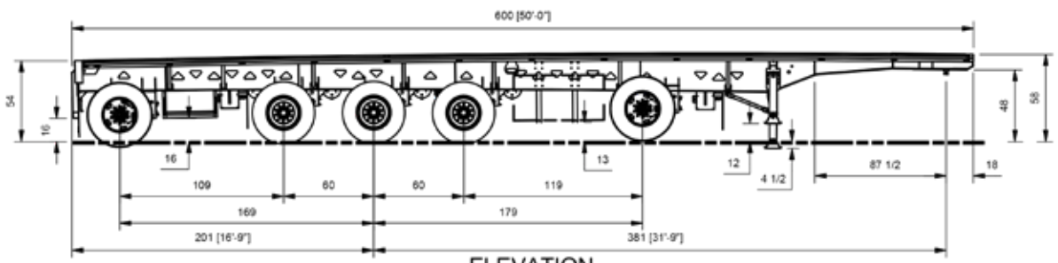
ELEVATION SCALE 1/75
