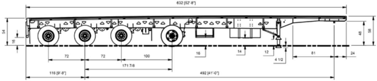
ELEVATION SCALE 1 / 75
