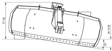
TILT POSITION ( LEFT OR RIGHT ) FRONT SCALE 1 / 50
