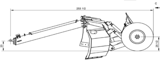
TILT POSITION ( LEFT OR RIGHT ) SIDE SCALE 1 / 50
