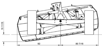
TILT POSITION ( LEFT OR RIGHT ) REAR SCALE 1 / 50
