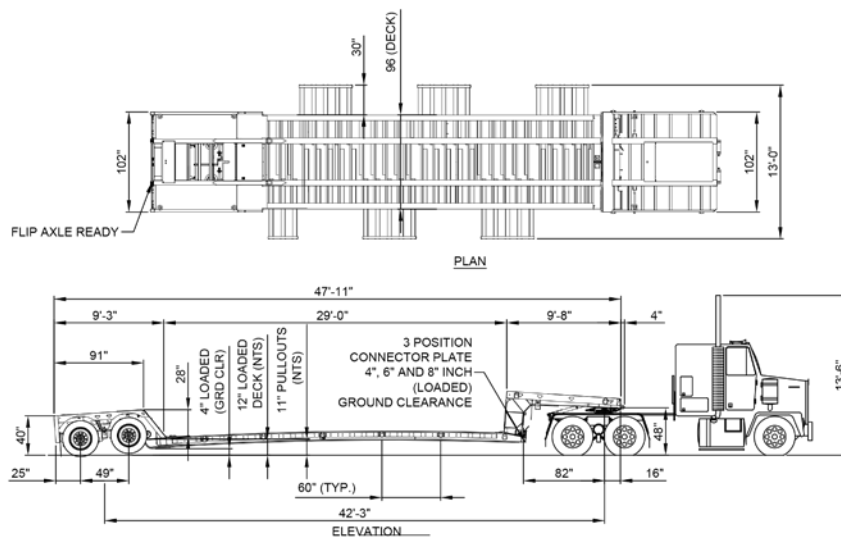
MODEL: 35MD2X48 AGULP 35TON MECHANICAL DETACHABLE GOOSENECK, 2 AXLE, 48 FT., AGRI, ULTRA LOW PRO NOTE: ALL DIMENSIONS ARE LOADED & NOMINAL
