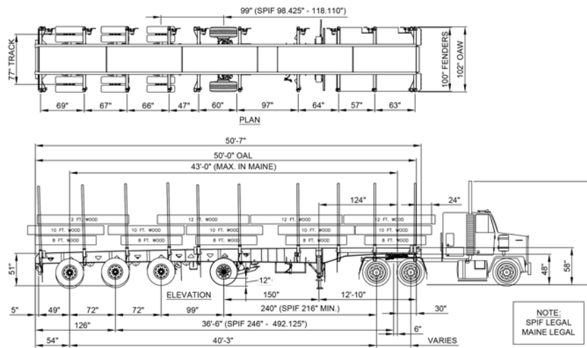
MODEL: 51LF4X5T NB V2016 51 FT. QUAD 5 TIER TAPER FRAME - NB
