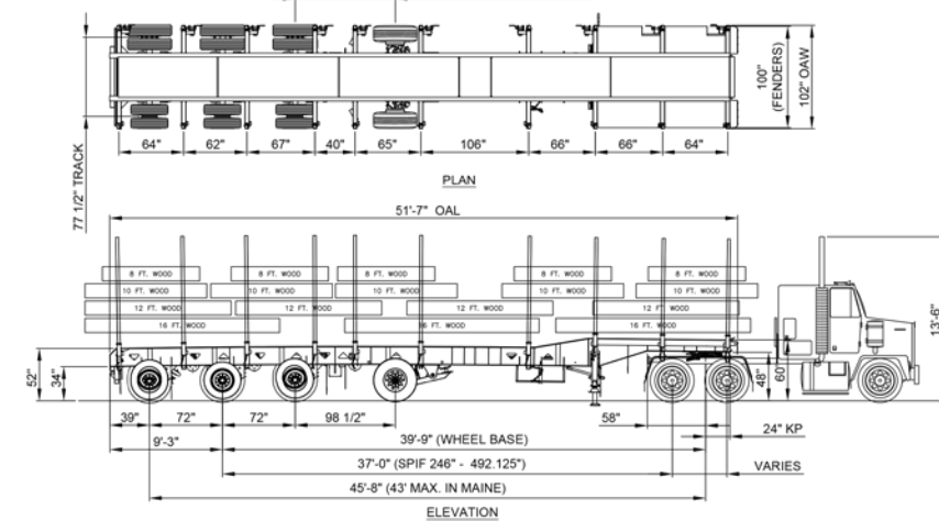
MODEL: 51LD4X5T NB V2016 51 FT. QUAD 5 TIER DROP FRAME - NB
