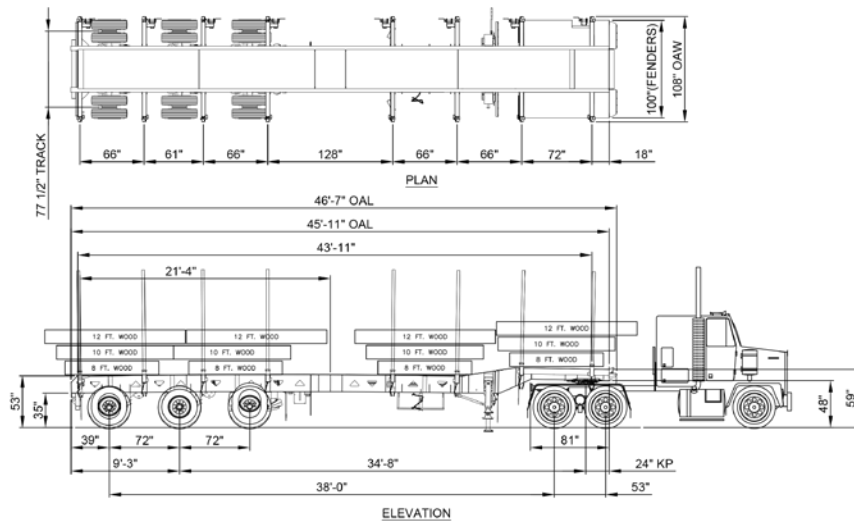
MODEL: 46LD3X4T NS V2016 46 FT. TRIDEM 4 TIER DROP FRAME - NS 99" (SPIF 98.425" - 118.110")
