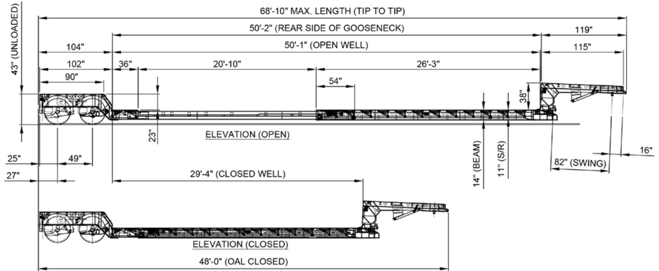
MODEL: 35MD2X EXT 35 TON MECHANICAL EXTENDABLE
