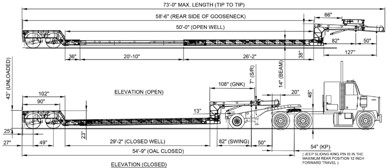
MODEL: 35MD2X EXT + FLIP EXT & JEEP DOLLY 35 TON MECHANICAL EXTENDABLE
