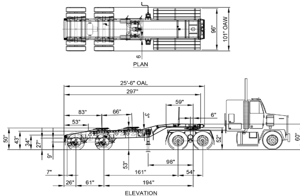
MODEL: 40JD2X OF 40 TON TANDEM OILFIELD NOTE: ALL DIMENSIONS ARE LOADED & NOMINAL.
