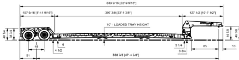
ELEVATION SCALE 1 / 100
