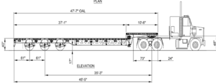
MODEL: 48HD3X 48' SINGLE DROP HIGHWAY TRAILER NOTE: ALL DIMENSIONS ARE NOMINAL
