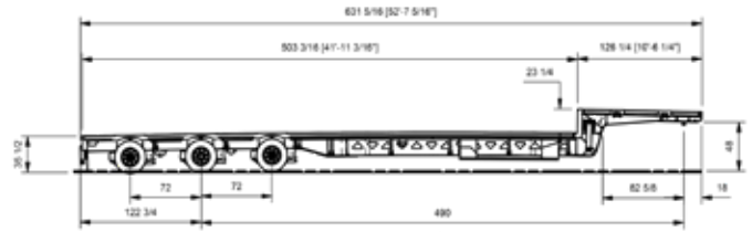
ELEVATION SCALE 1 / 100
