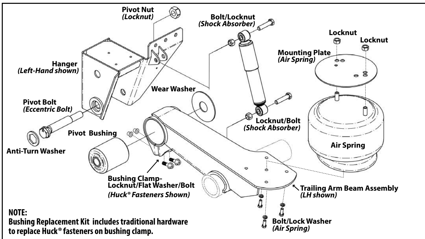
Figure 7. 240-30K Overslung Suspension Components Refer to the suspension model engineering drawing for the individual component part number.
