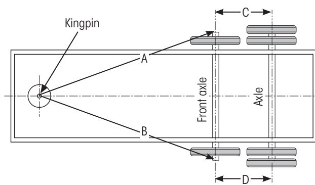
Figure 13: Measurements to check axle-to-axle alignment
