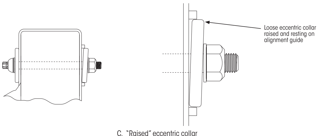
Figure 35: QUIK-ALIGN® Pivot connection hardware positioning
