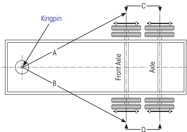
Figure 22: Axle alignment measurements
