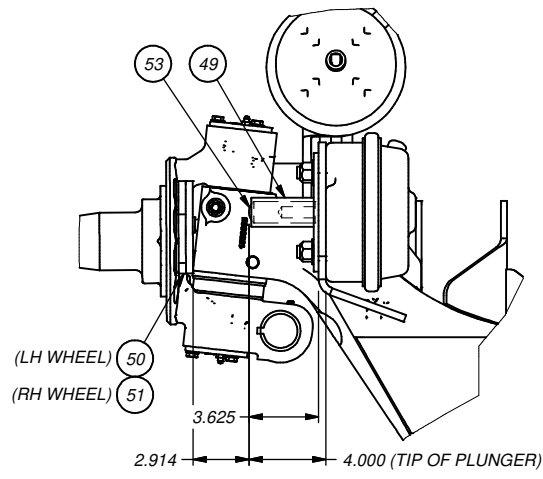
PLUNGER DETAIL
